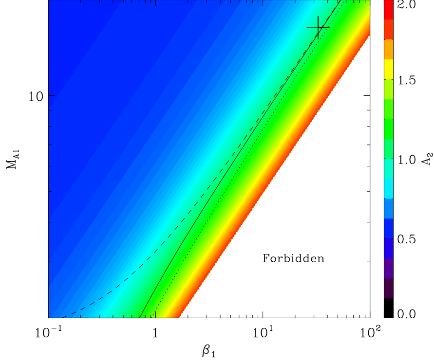
Figure 6-2: Temperature anisotropy downstream of a parallel shock with r_s = 3 and A_1 = 1 as a function of \beta_1 and M_{A1} . Same format as Figure 1. Regions below the mirror/ion cyclotron threshold are unstable to the mirror/ion cyclotron mode and regions above the firehose onset are unstable to the firehose instability.
