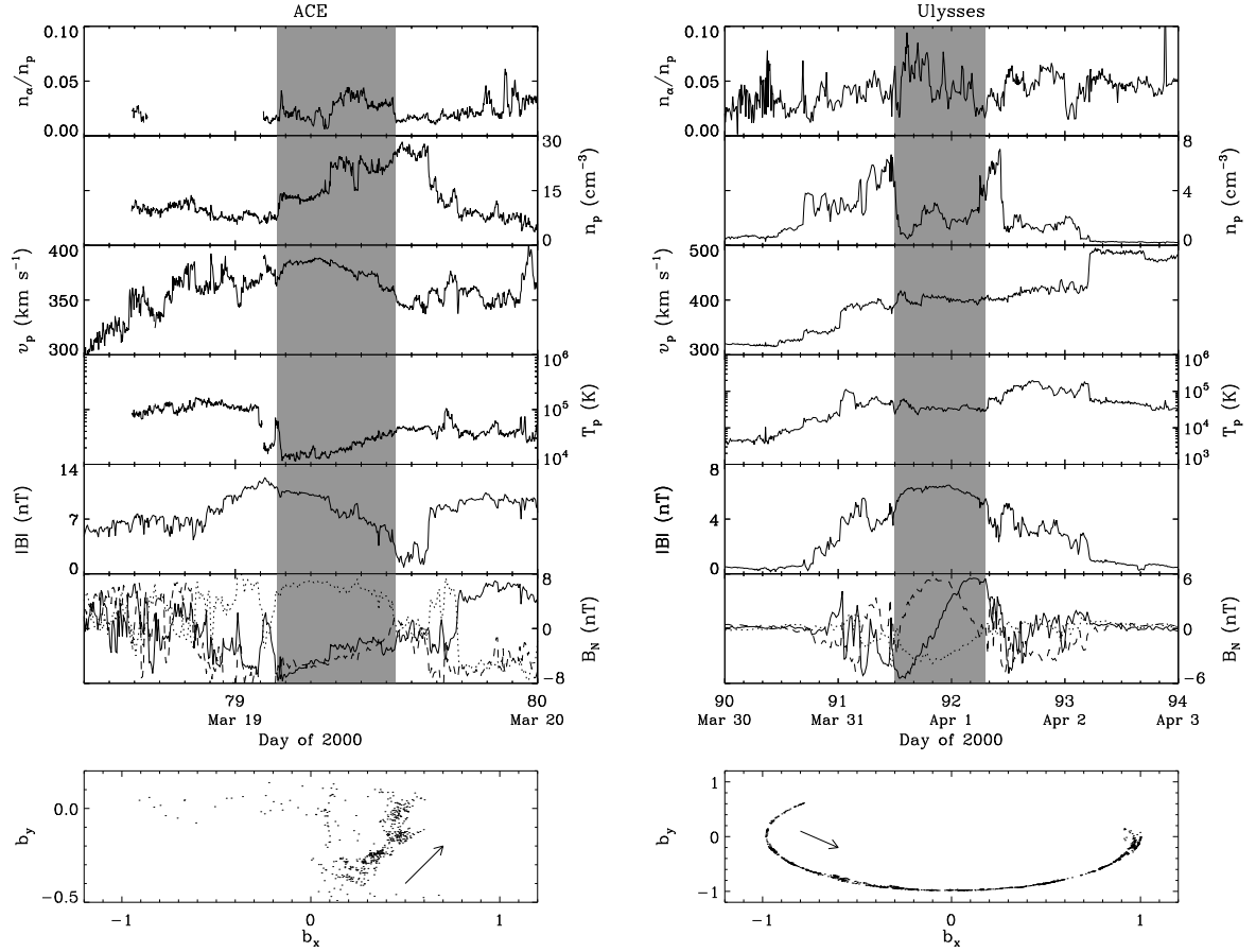
Figure 3-3: Solar wind plasma and magnetic field parameters for Case 2 in Table 3.1. Same format as Figure 3-2.
