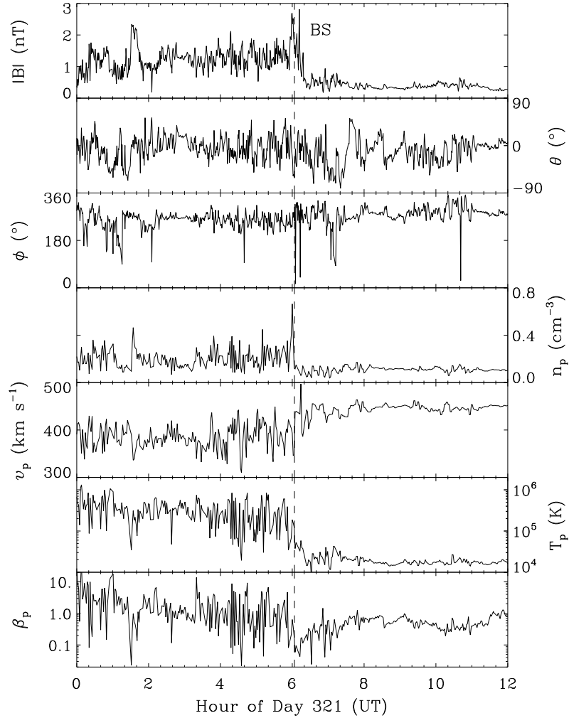
Figure 6-4: Outbound crossing of Saturn's bow shock. Quasi-parallel. The bow shock crossing occurs at 77.9R_S in Saturnian system.
