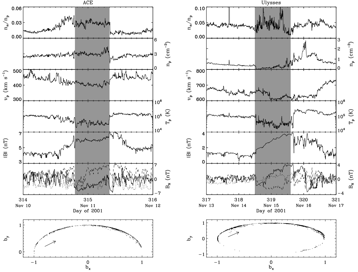
Figure 3-4: Solar wind plasma and magnetic field parameters for Case 3 in Table 3.1. Same format as Figure 3-2.
