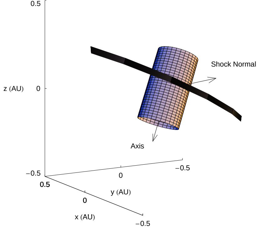
Figure 5-5: A 3-D rendering of the MC in GSE coordinates. Arrows indicate the axis orientation and shock normal, respectively. The belt around the flux tube approximates the shock surface.
